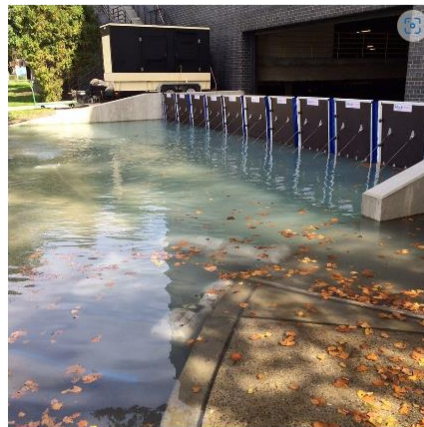
FloodWall
